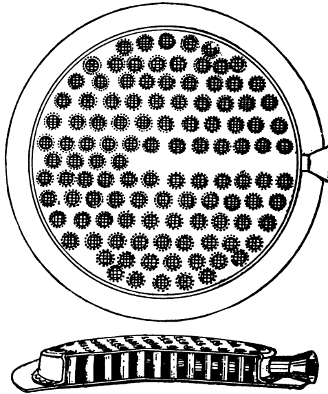
FIG. 361.—Plan and Part Section of a Typical Gasoline Burner for Steam Carriage Use.
